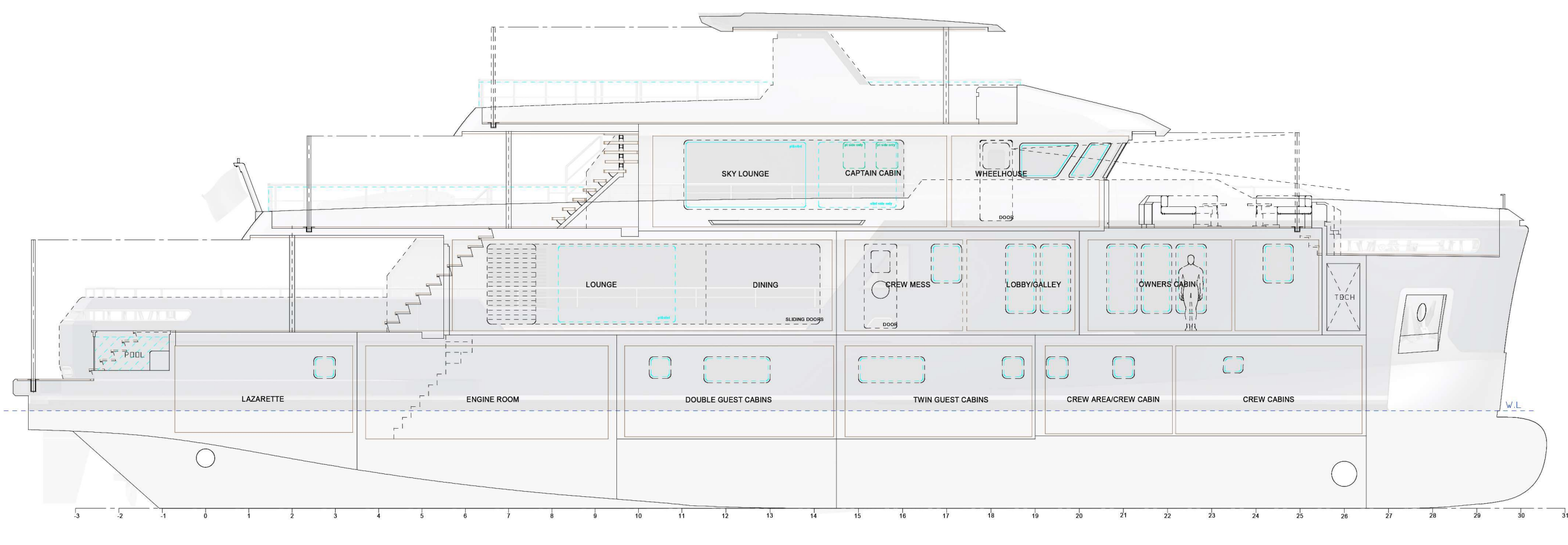
DESIGN SECTION
