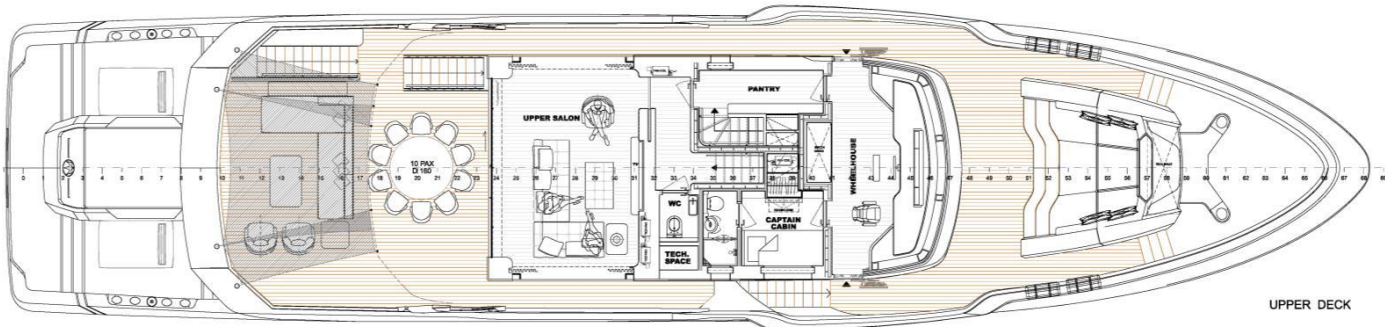
UD ALTERNATIVE LAYOUT: VERANDA OPTION
