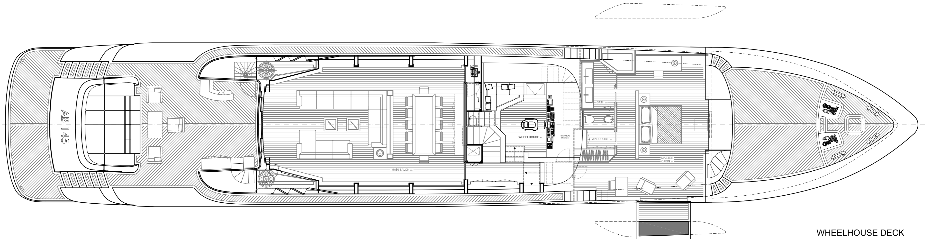
WHEELHOUSE DECK
